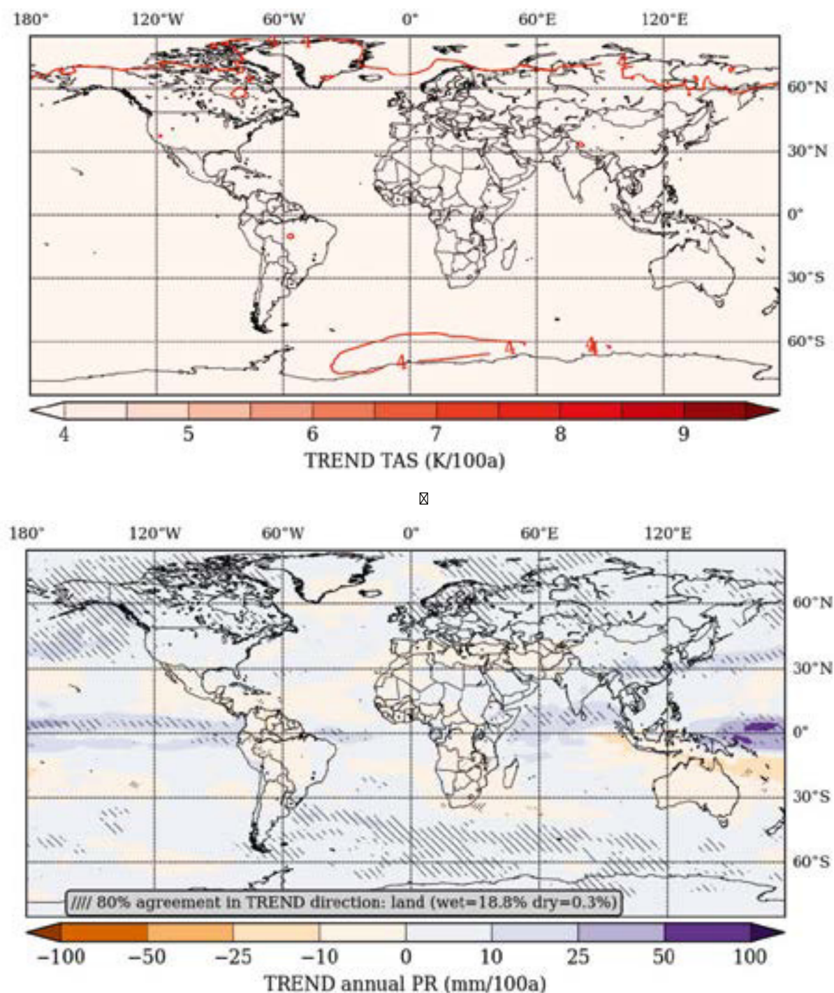
Figure 6: Mean trend in average annual temperature and average annual precipitation until the end of this century under RCP2.6 (low radioactive forcing and temperature increase) – Data processed at Potsdam Institute for Climate Impact Research.
