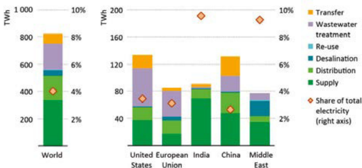
Figure 35: Electricity consumption in the water sector by process and region, 2014, Source: IEA, 2016.
